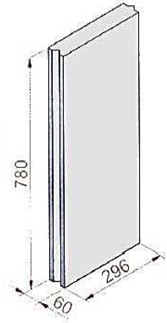
Quickboard 780 R8631 780 005
